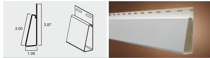
WINDOW CASING TRIM
