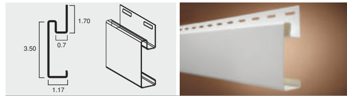
3-1/2" WINDOW & DOOR TRIM
