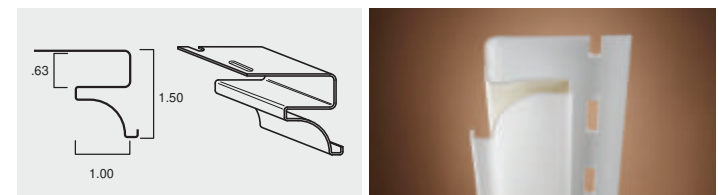
CROWN MOLDING
