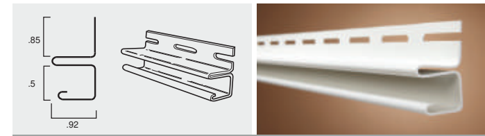
1/2" F-CHANNEL
