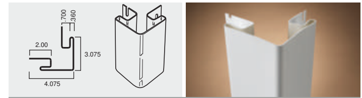
3" OUTSIDE CORNER POST - 12'
