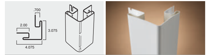
3" OUTSIDE CORNER POST - 10'
