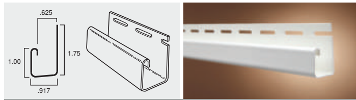
5/8" J-CHANNEL
