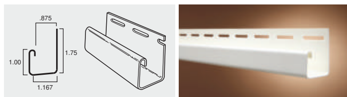
7/8" J-CHANNEL
