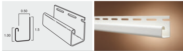
1/2" J-CHANNEL - 1" FACE
