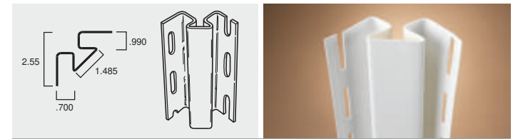
INSIDE CORNER POST
