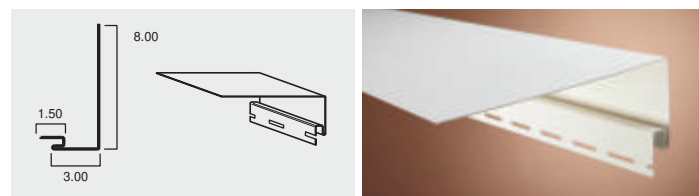
RECESSED WINDOW & DOOR TRIM
