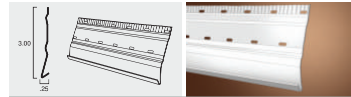
GALVANIZED STARTER STRIP
