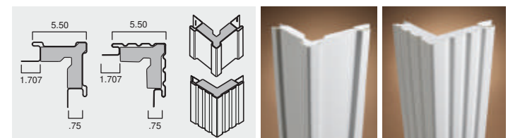
TRADITIONAL OR FLUTED 5-1/2" OUTSIDE CORNER POST - 20'
